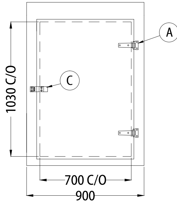
EXTERNAL VIEW ON FRONT WALL
